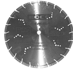
14" x .125 1" UNIVERSAL CONCRETE/ASPHALT BLADE
